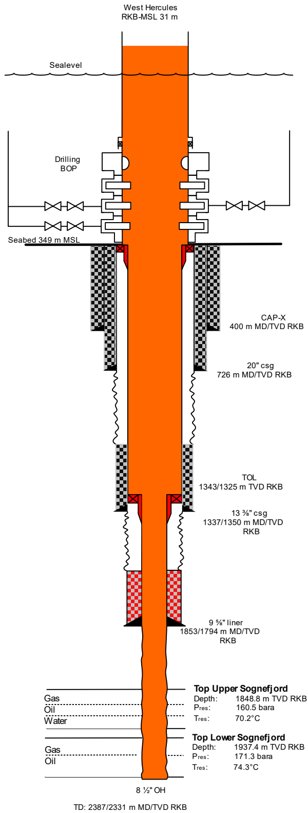
Figure 2: Schematics for the Blasto well
