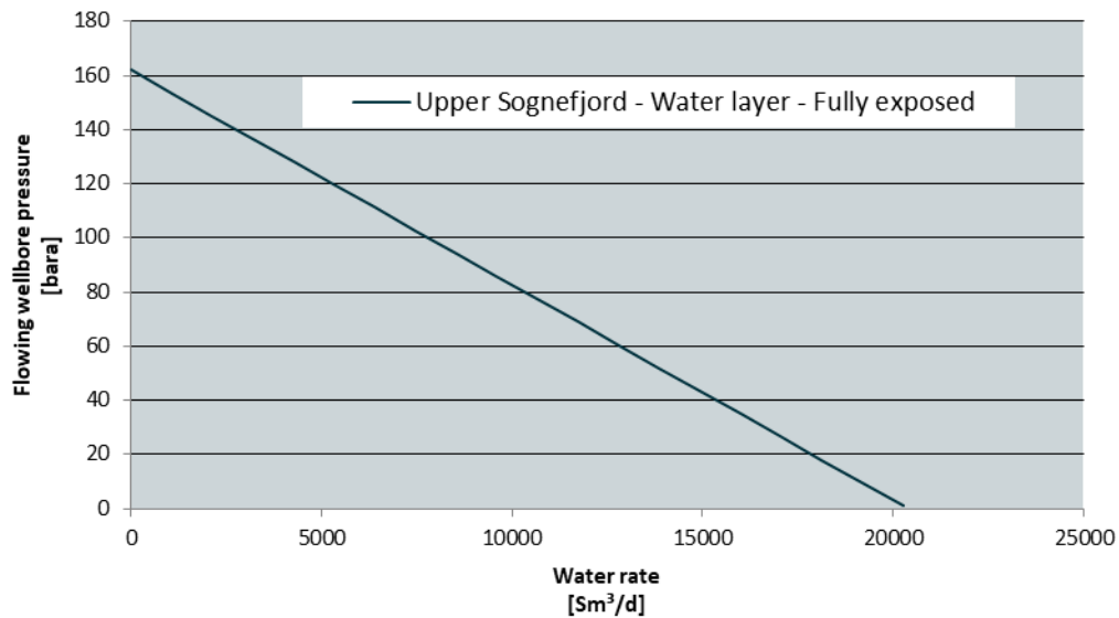
Figure 5: Water inflow performance
