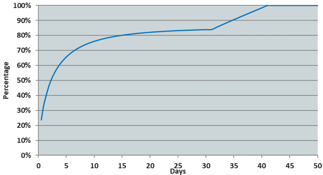
Figure 11: Reliability presentation of all kill actions when combined for a surface release
