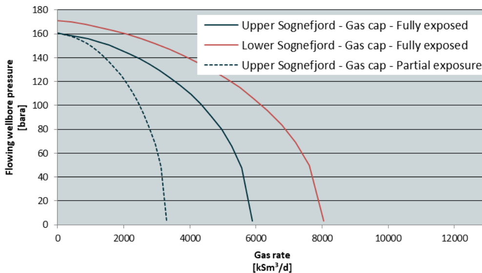
Figure 3: Gas inflow performance
