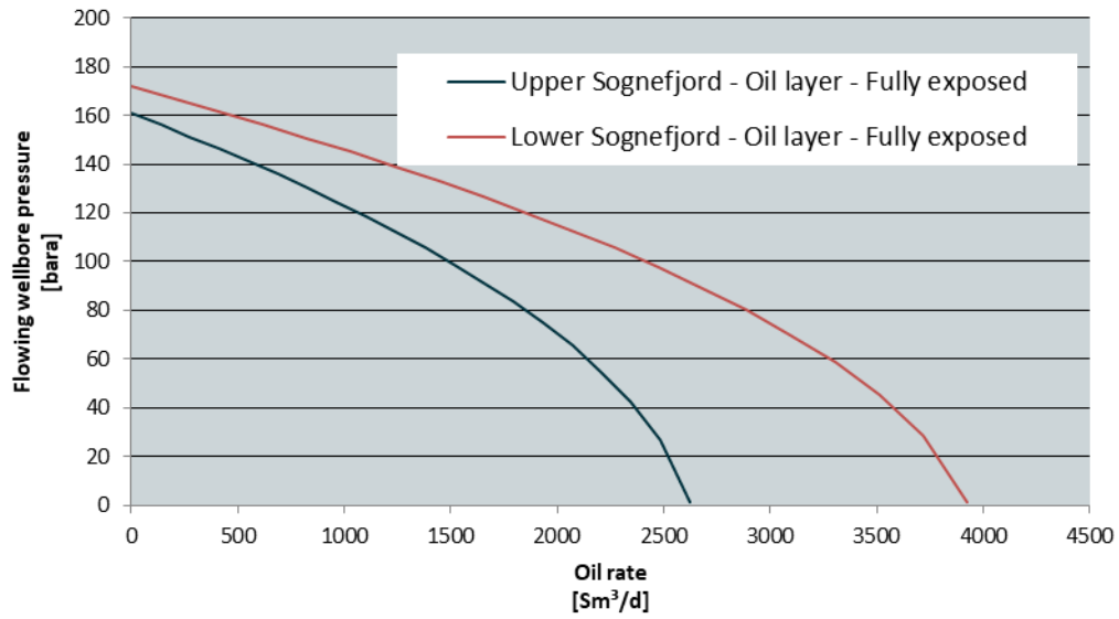
Figure 4: Oil inflow performance
